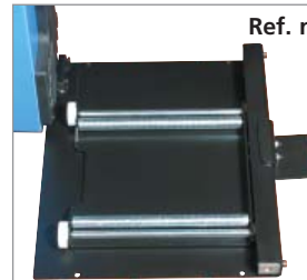
Roller board for ergonomic bead breaking
